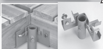
"C" Inside Corner Bracket
